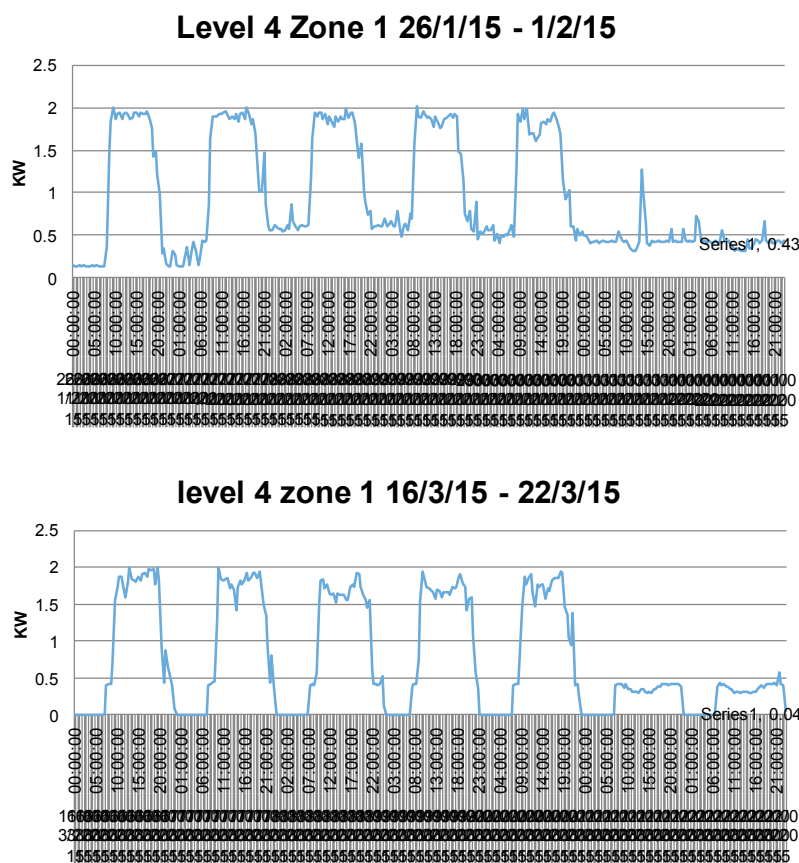
Figure 8. Weekly Plot of Lighting Energy Consumption before and after application of the ECM.
